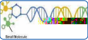
DNA
